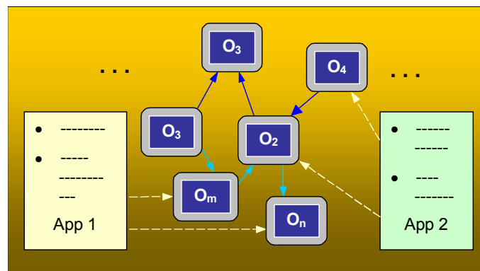
Figure 2 - Semantic markup provides mappings between Web pages and ontologies (O i - ontologies)
