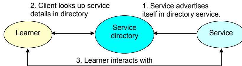
Figure 3 – Service-oriented architecture of educational Web servers
