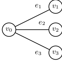
Figure 1: A CVC instance: c(v_0) = 3 and \ell(e_i) = 2 for i \in \{1, 2, 3\} . If the demands are separable two copies of v_0 are sufficient to cover the three edges, but if the demands are inseparable three copies of v_0 are needed.
