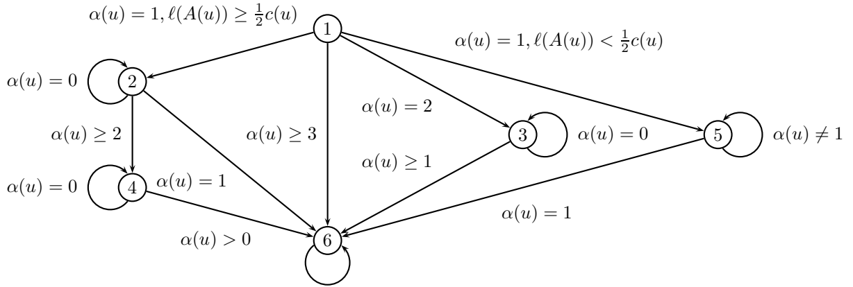
(b) Possible transitions between the conditions.
