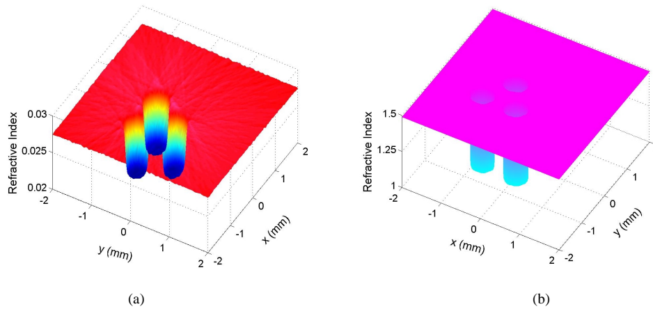
Fig. 3. Three-hole Polymer HFP tomography plots (a) Three dimensional display of the measured refractive index profile of a polymer filled holey fibre preform (bottom view) (b) Three dimensional display of the refractive index profile of the polymer HFP.
