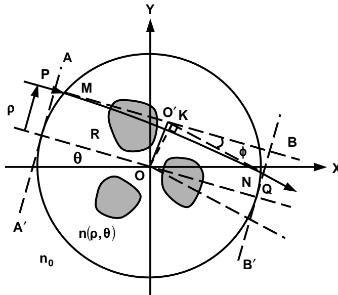
Fig. 1. Ray trajectory in a Filled Holey Fiber preform (FHFP) cross section
