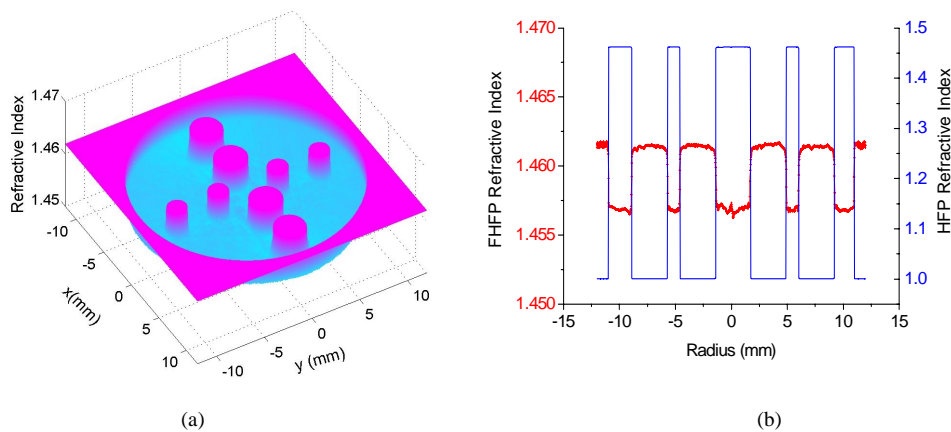
Fig. 2. Eight-hole silica HFP tomography plots: (a) Refractive index distribution of three-dimensional display of FHFP; (b) Cross-section display of HFP.
