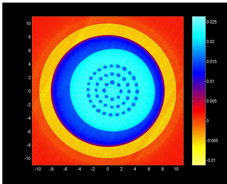
Fig. 4. Two-dimensional display of the refractive index profile of the three-ring 48 holes polymer FHFP.
