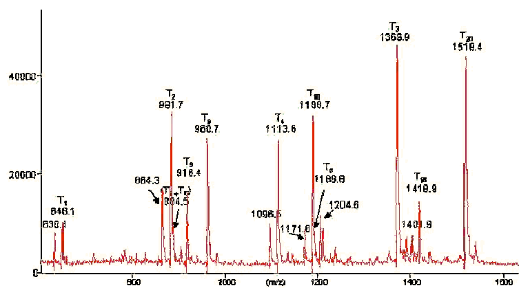
Maldi ToF mass spectrum of the tryptic digest of a high molecular weight (85,000) glutenin (DVF10)
