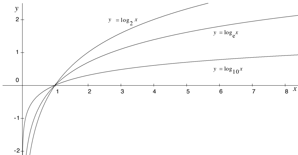
Figure 7: Graph of f(x) = \log_b x for various values of b .
