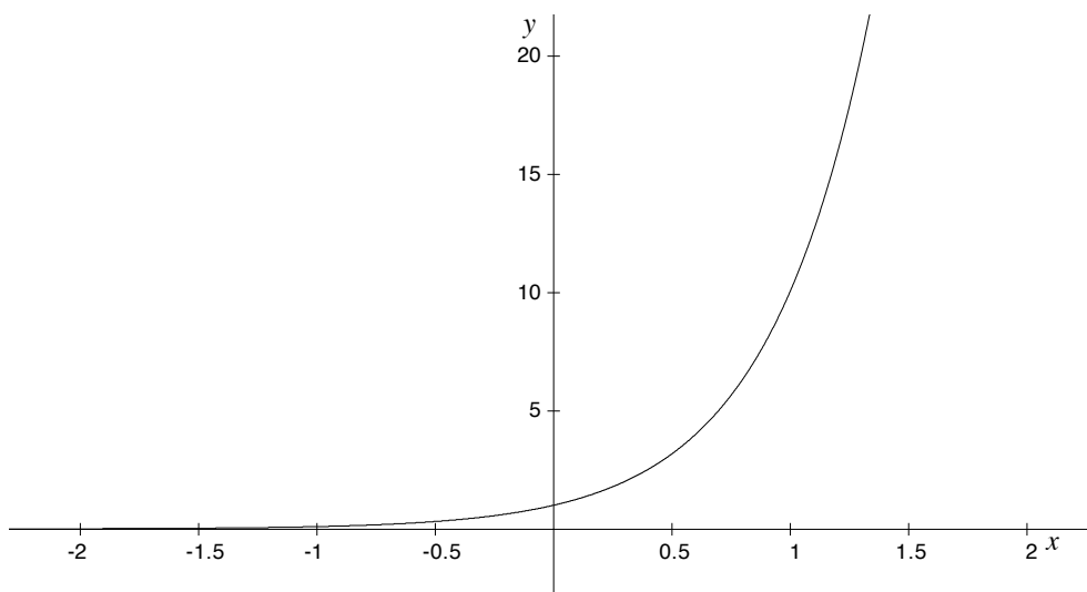
Figure 5: Graph of f(x) = 10^x
