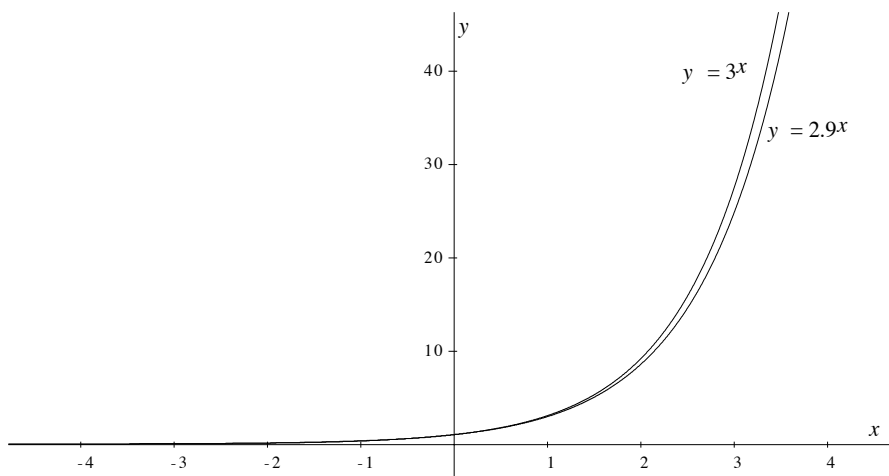
Figure 10: Graphs of y = 3^x and y = 2.9^x .
