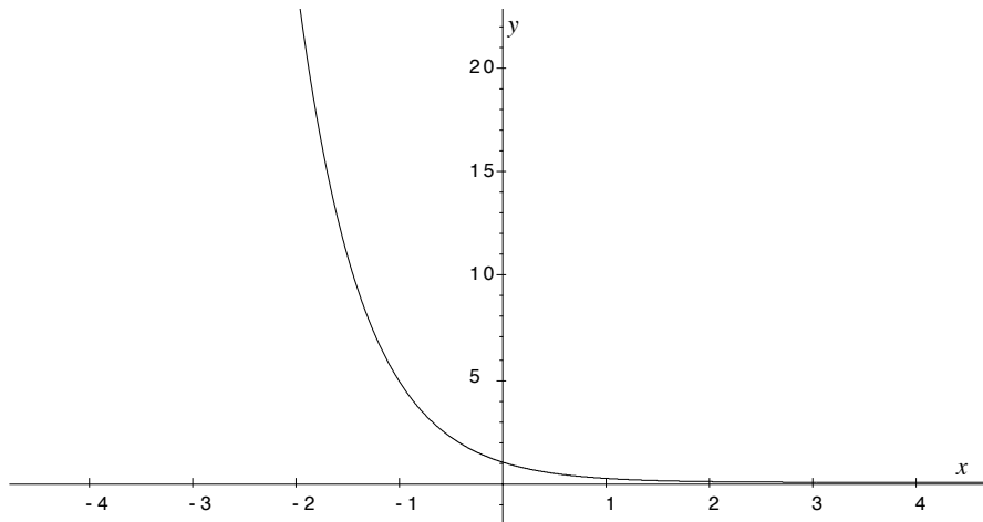
Figure 9: Graph of y = 5^{-x} .
