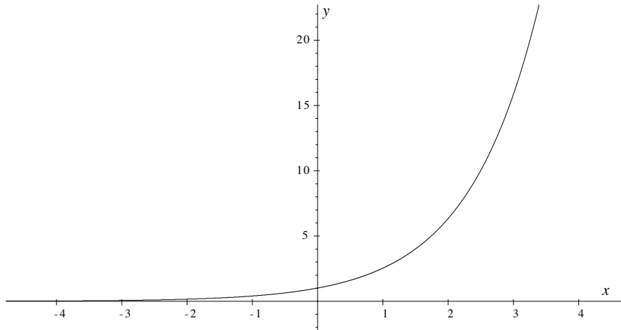
Figure 8: Graph of y = 2.5^x .
