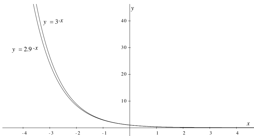
Figure 11: Graphs of y = 3^{-x} and y = 2.9^{-x} .
