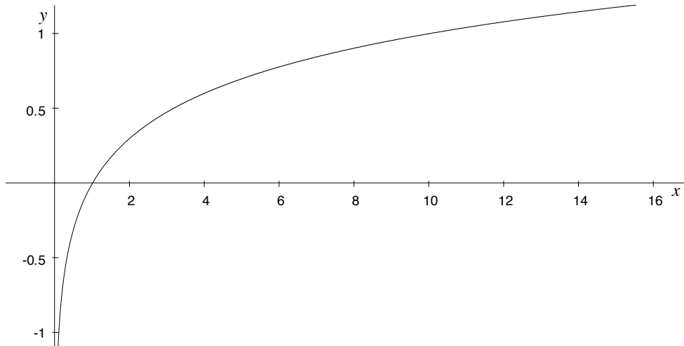
Figure 6: Graph of f(x) = \log_{10} x
