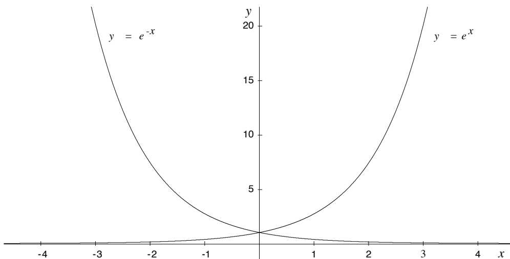
Figure 4: Graphs of e^x and e^{-x} .
